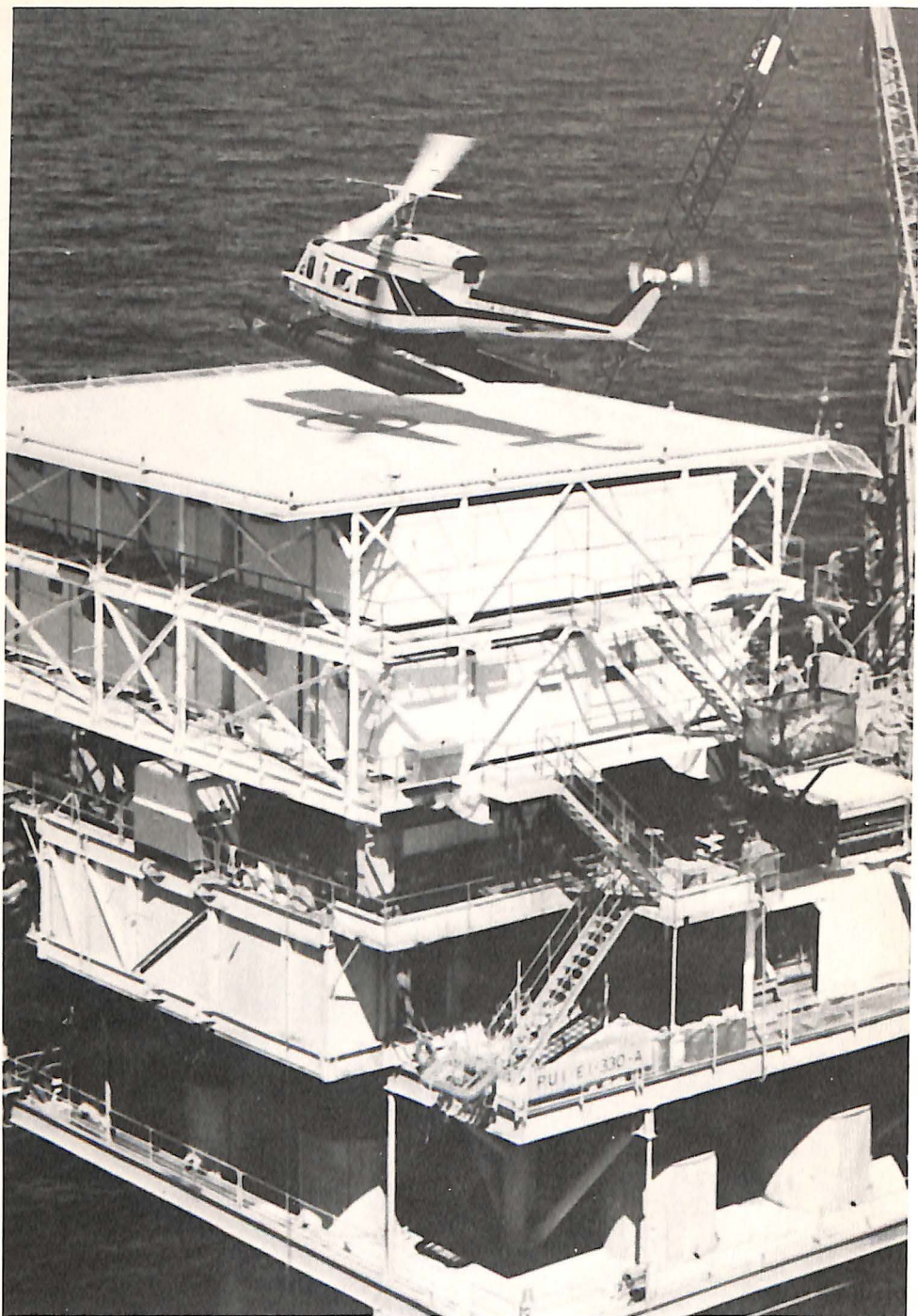
Helicopters have been serving the off-shore oil industry for more than 25 years, moving crews, supplies, parts. The farther companies move off-shore, the greater is their need for helicopters. Here a Bell twin-engine 212 helicopter serves as the daily "bus" for oil crews to an oil production platform in the Gulf of Mexico.
