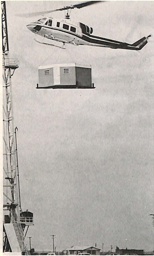
The Bell Big Lifter -- the 214B helicopter -- demonstrates its capability of lifting more than 7,000 pounds.
