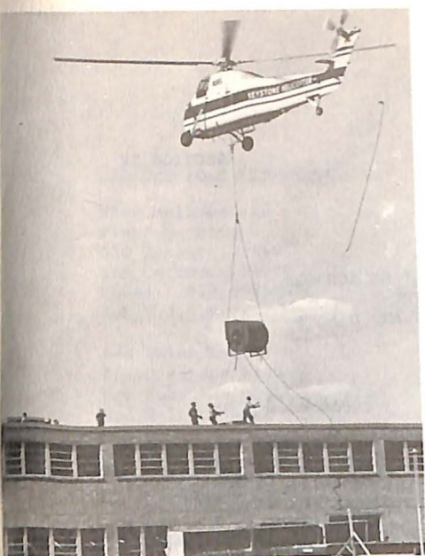
For heavy lift jobs -- construction -- these Keystone and St. Louis Airways helicopters show how they can cut time and costs.
