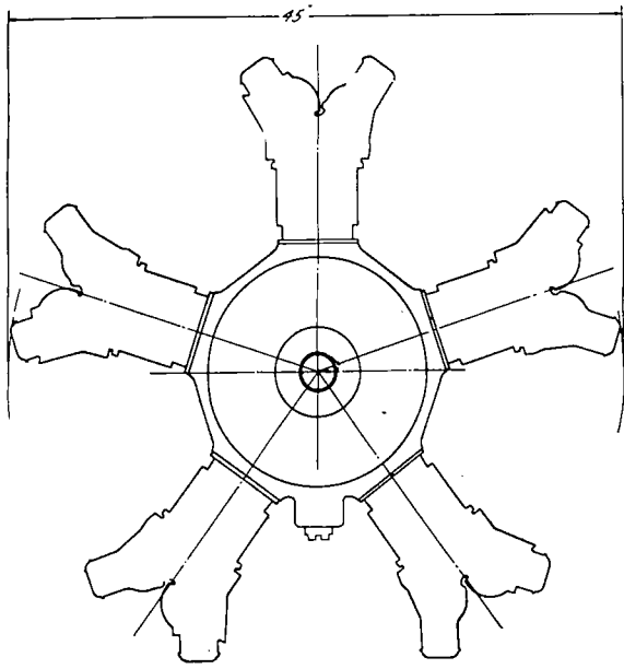
WRIGHT AERONAUTICAL CORPORATION PATERSON, N. J. "WHIRLWIND" 5 CYLINDERS AIRCOOLED STANDARD 150 B.H.P. AT 1800 R.P.M. WEIGHT DRY 370 LBS.
