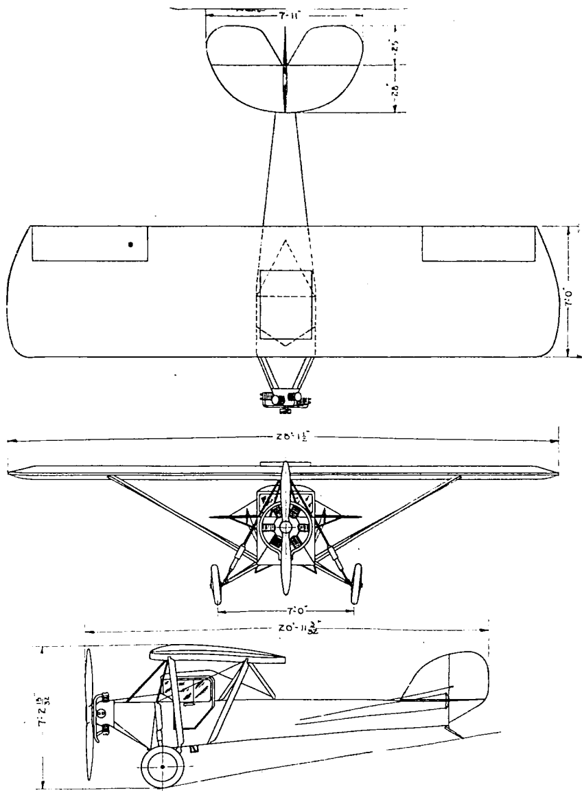
G. ELIAS & BRO., INC. BUFFALO, N. Y. CABIN MONOPLANE "EC-1" ENGINE—ANZANI 80 H.P.
