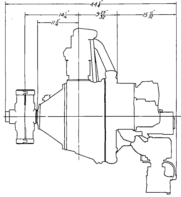
WRIGHT AERONAUTICAL CORPORATION PATERSON, N. J. "WHIRLWIND" 5 CYLINDERS AIRCOOLED STANDARD 150 B.H.P. AT 1800 R.P.M. WEIGHT DRY 370 LBS.
